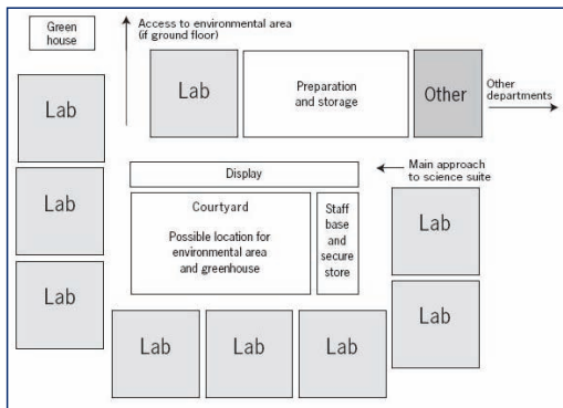
■ Courtyard Plan.
